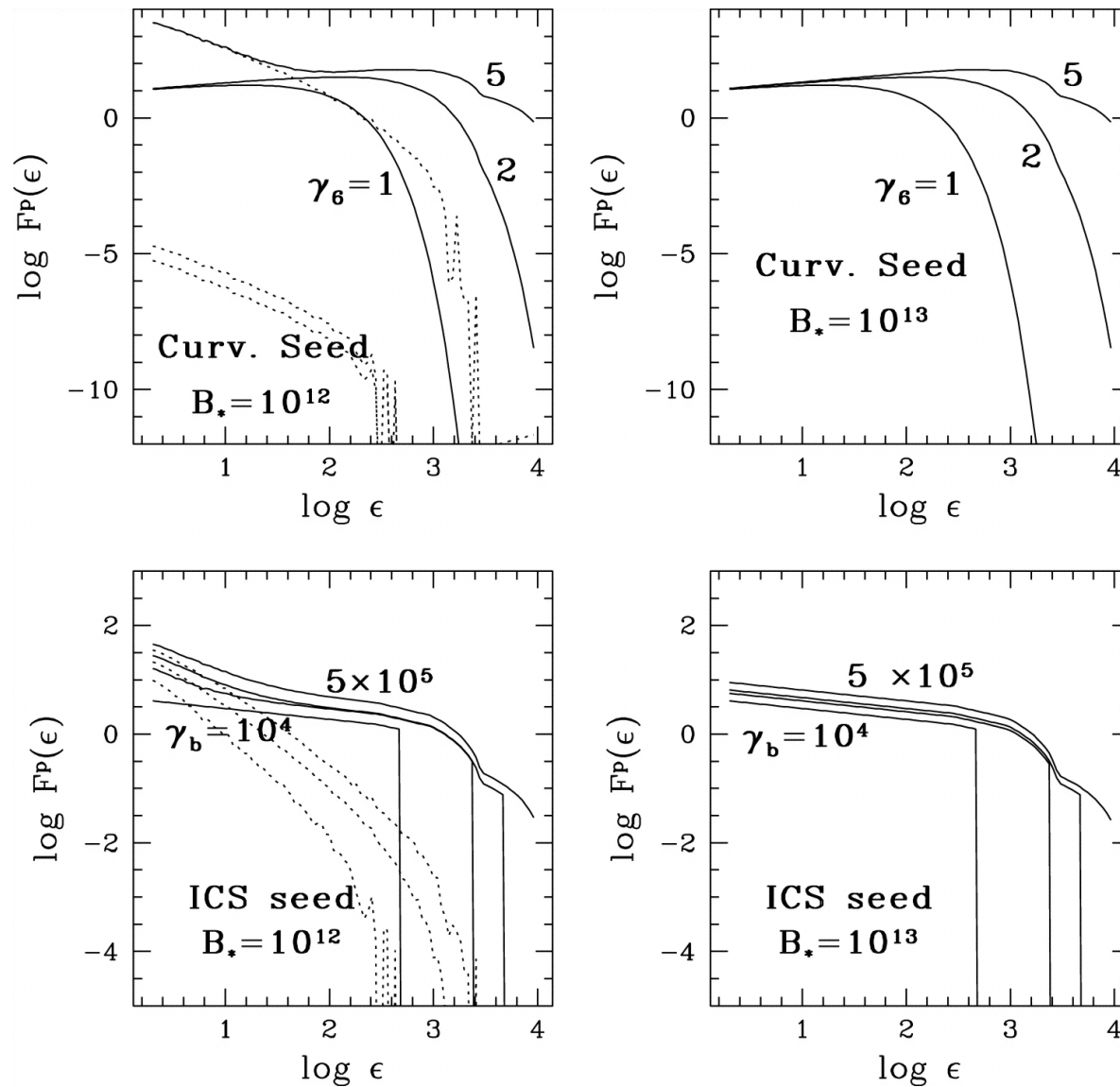
Fig. 10. from Pair Creation in the Pulsar Magnetosphere Arendt & Eilek 2002 ApJ 581 451 doi:10.1086/344133 https://dx.doi.org/10.1086/344133 © 2002. The American Astronomical Society. All rights reserved. Printed in U.S.A.
