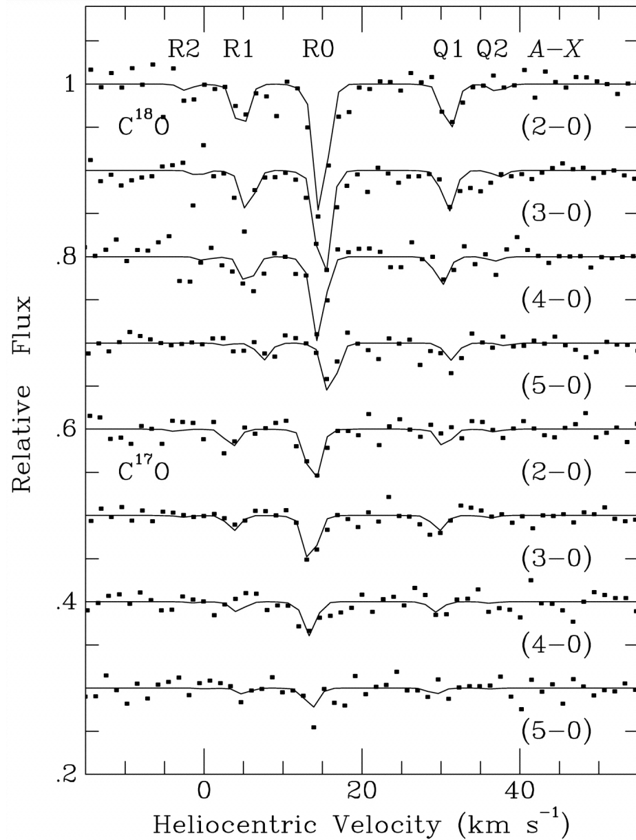
Fig. 1. from Ultraviolet Detection of Interstellar ^{12}\text{C}^{17}\text{O} and the CO Isotopomeric Ratios toward X Persei Sheffer, Lambert, & Federman 2002 ApJL 574 L171 doi:10.1086/342501 https://dx.doi.org/10.1086/342501
