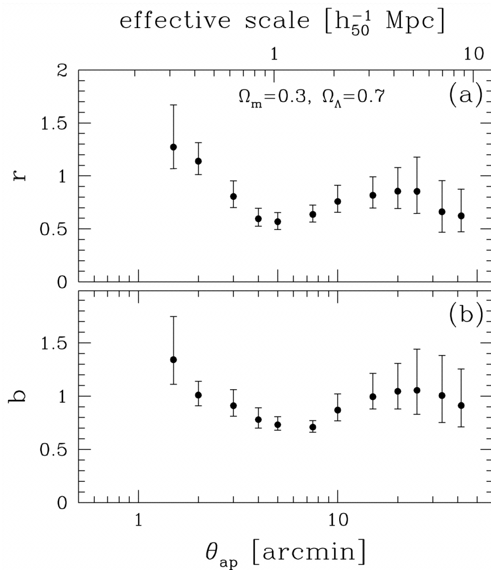
Fig. 5. from Weak Lensing Study of Galaxy Biasing Hoekstra et al. 2002 ApJ 577 604 doi:10.1086/342228 https://dx.doi.org/10.1086/342228 © 2002. The American Astronomical Society. All rights reserved. Printed in U.S.A.
