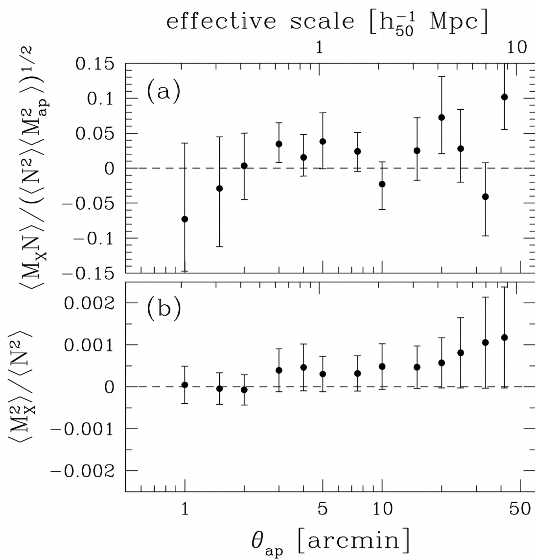
Fig. 4. from Weak Lensing Study of Galaxy Biasing Hoekstra et al. 2002 ApJ 577 604 doi:10.1086/342228 https://dx.doi.org/10.1086/342228 © 2002. The American Astronomical Society. All rights reserved. Printed in U.S.A.
