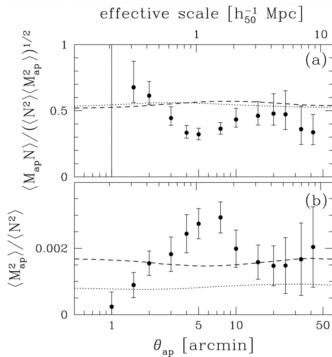
Fig. 3. from Weak Lensing Study of Galaxy Biasing Hoekstra et al. 2002 ApJ 577 604 doi:10.1086/342228 https://dx.doi.org/10.1086/342228 © 2002. The American Astronomical Society. All rights reserved. Printed in U.S.A.
