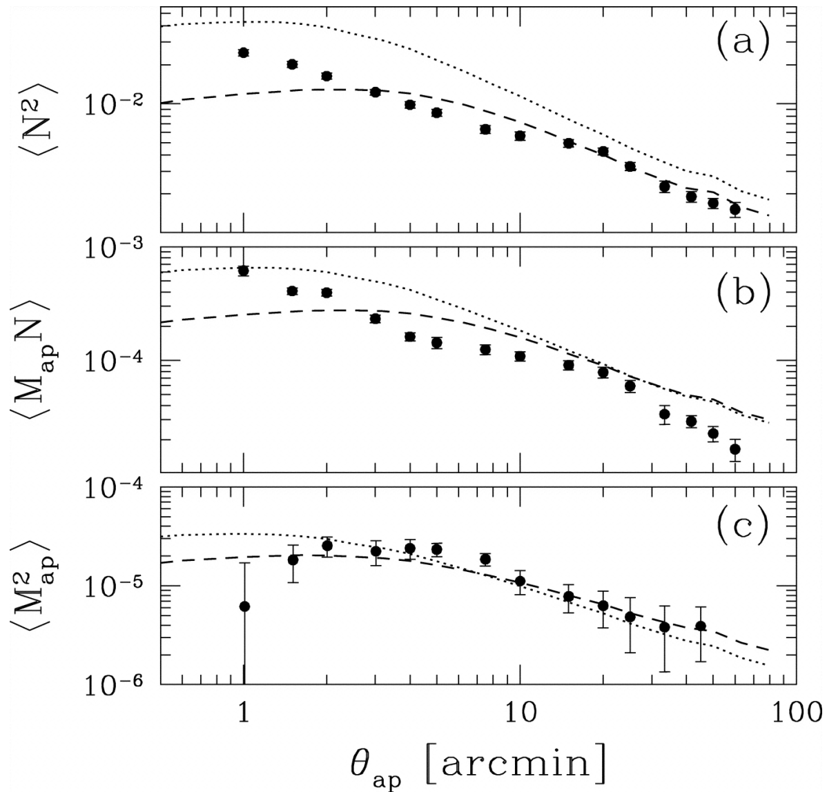
Fig. 2. from Weak Lensing Study of Galaxy Biasing Hoekstra et al. 2002 ApJ 577 604 doi:10.1086/342228 https://dx.doi.org/10.1086/342228 © 2002. The American Astronomical Society. All rights reserved. Printed in U.S.A.
