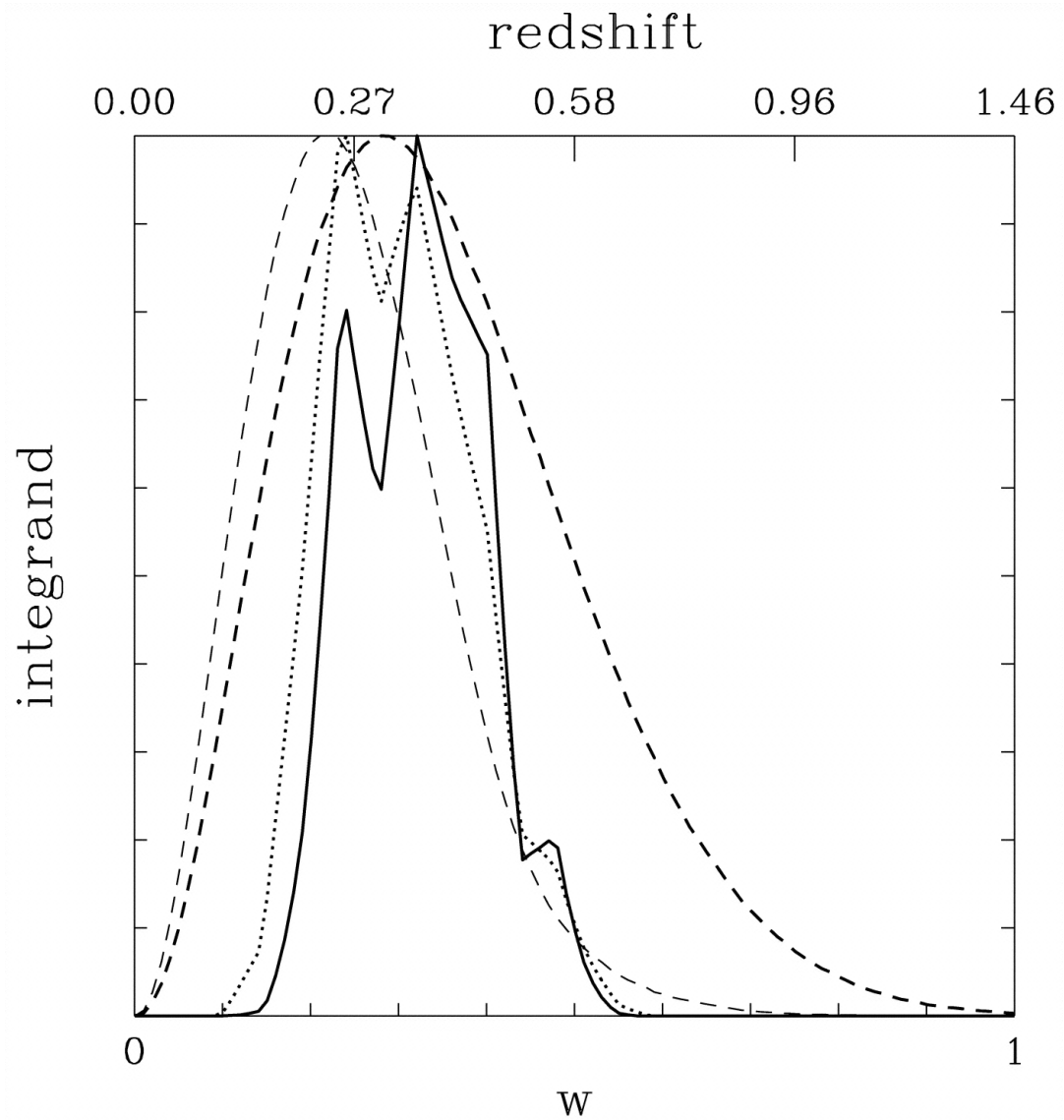
Fig. 1. from Weak Lensing Study of Galaxy Biasing Hoekstra et al. 2002 ApJ 577 604 doi:10.1086/342228 https://dx.doi.org/10.1086/342228 © 2002. The American Astronomical Society. All rights reserved. Printed in U.S.A.
