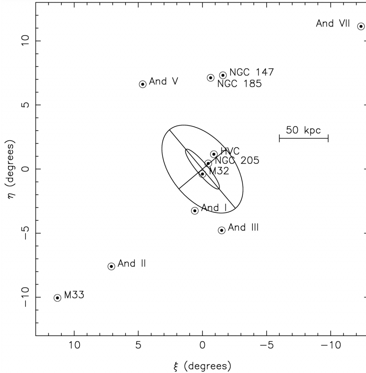
Fig. 8. from Evidence for Stellar Substructure in the Halo and Outer Disk of M31 Ferguson et al. 2002 AJ 124 1452 doi:10.1086/342019 https://dx.doi.org/10.1086/342019 © 2002. The American Astronomical Society. All rights reserved. Printed in U.S.A.
