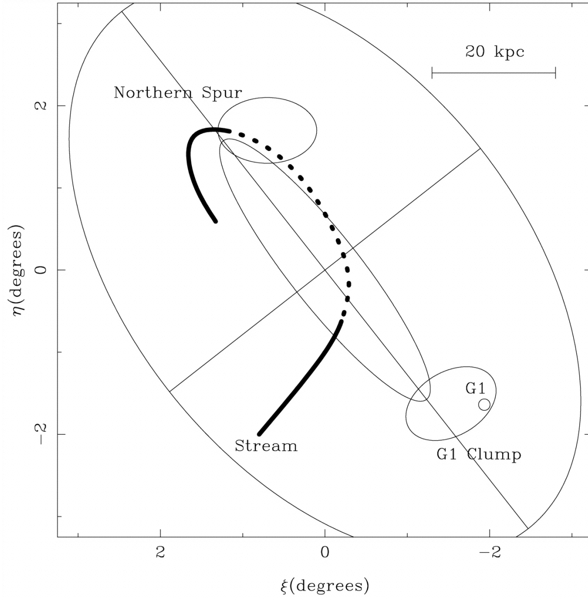
Fig. 7. from Evidence for Stellar Substructure in the Halo and Outer Disk of M31 Ferguson et al. 2002 AJ 124 1452 doi:10.1086/342019 https://dx.doi.org/10.1086/342019 © 2002. The American Astronomical Society. All rights reserved. Printed in U.S.A.
