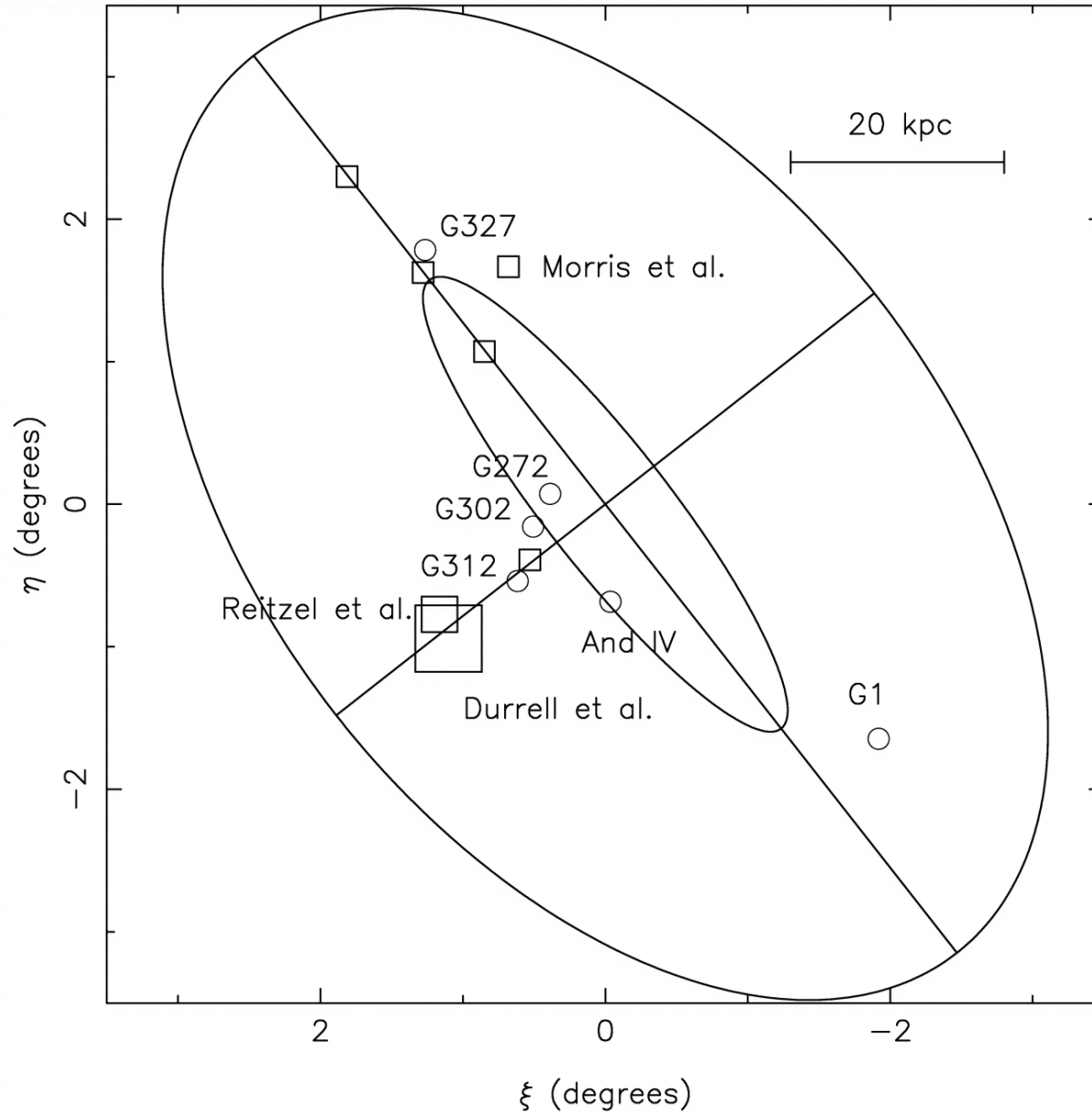
Fig. 6. from Evidence for Stellar Substructure in the Halo and Outer Disk of M31 Ferguson et al. 2002 AJ 124 1452 doi:10.1086/342019 https://dx.doi.org/10.1086/342019 © 2002. The American Astronomical Society. All rights reserved. Printed in U.S.A.
