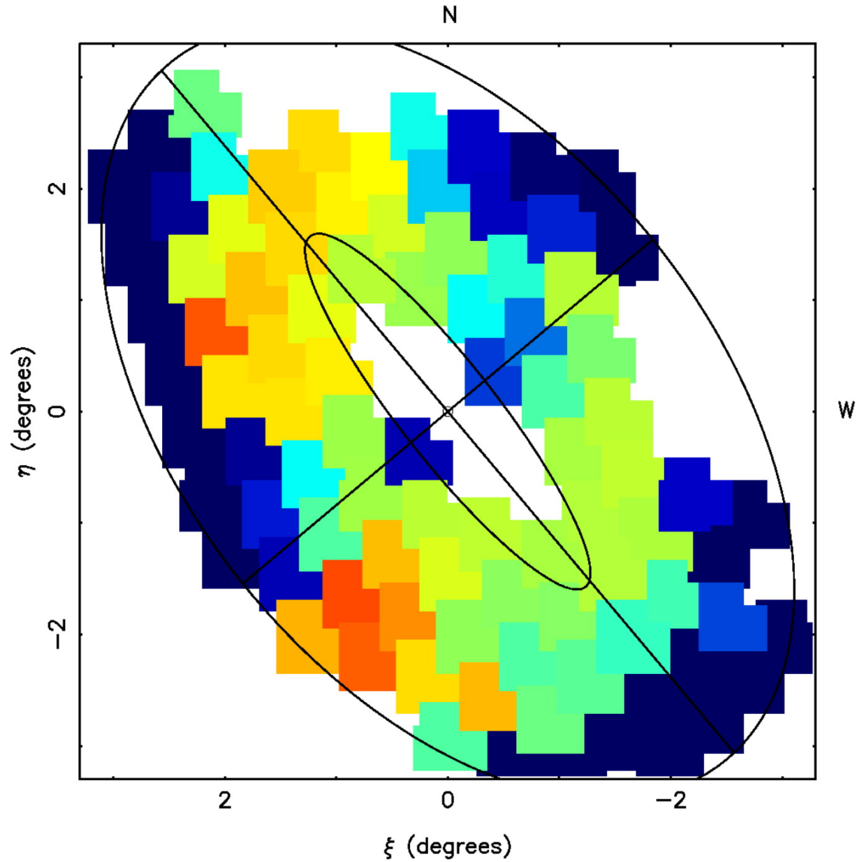
Fig. 5. from Evidence for Stellar Substructure in the Halo and Outer Disk of M31 Ferguson et al. 2002 AJ 124 1452 doi:10.1086/342019 https://dx.doi.org/10.1086/342019 © 2002. The American Astronomical Society. All rights reserved. Printed in U.S.A.
