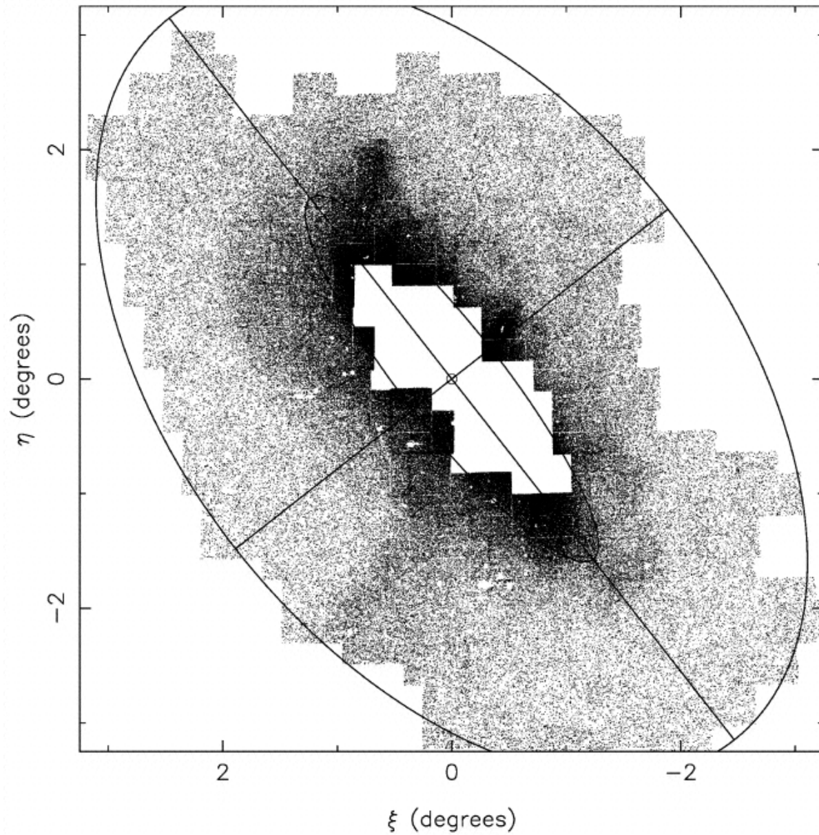
Fig. 2. from Evidence for Stellar Substructure in the Halo and Outer Disk of M31 Ferguson et al. 2002 AJ 124 1452 doi:10.1086/342019 https://dx.doi.org/10.1086/342019 © 2002. The American Astronomical Society. All rights reserved. Printed in U.S.A.
