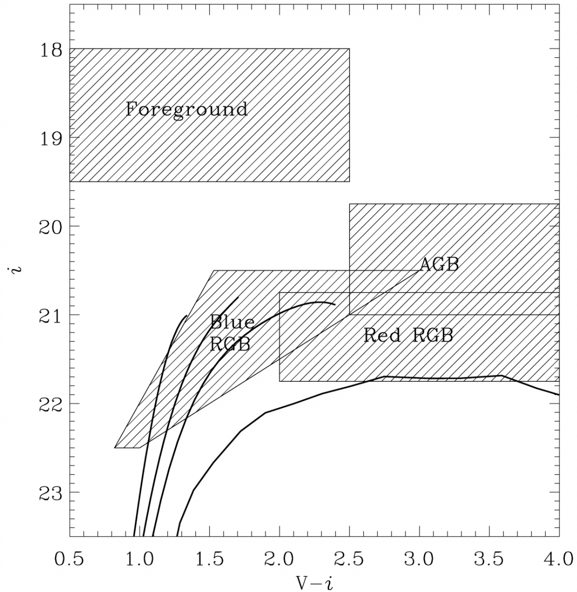
Fig. 1. from Evidence for Stellar Substructure in the Halo and Outer Disk of M31 Ferguson et al. 2002 AJ 124 1452 doi:10.1086/342019 https://dx.doi.org/10.1086/342019 © 2002. The American Astronomical Society. All rights reserved. Printed in U.S.A.
