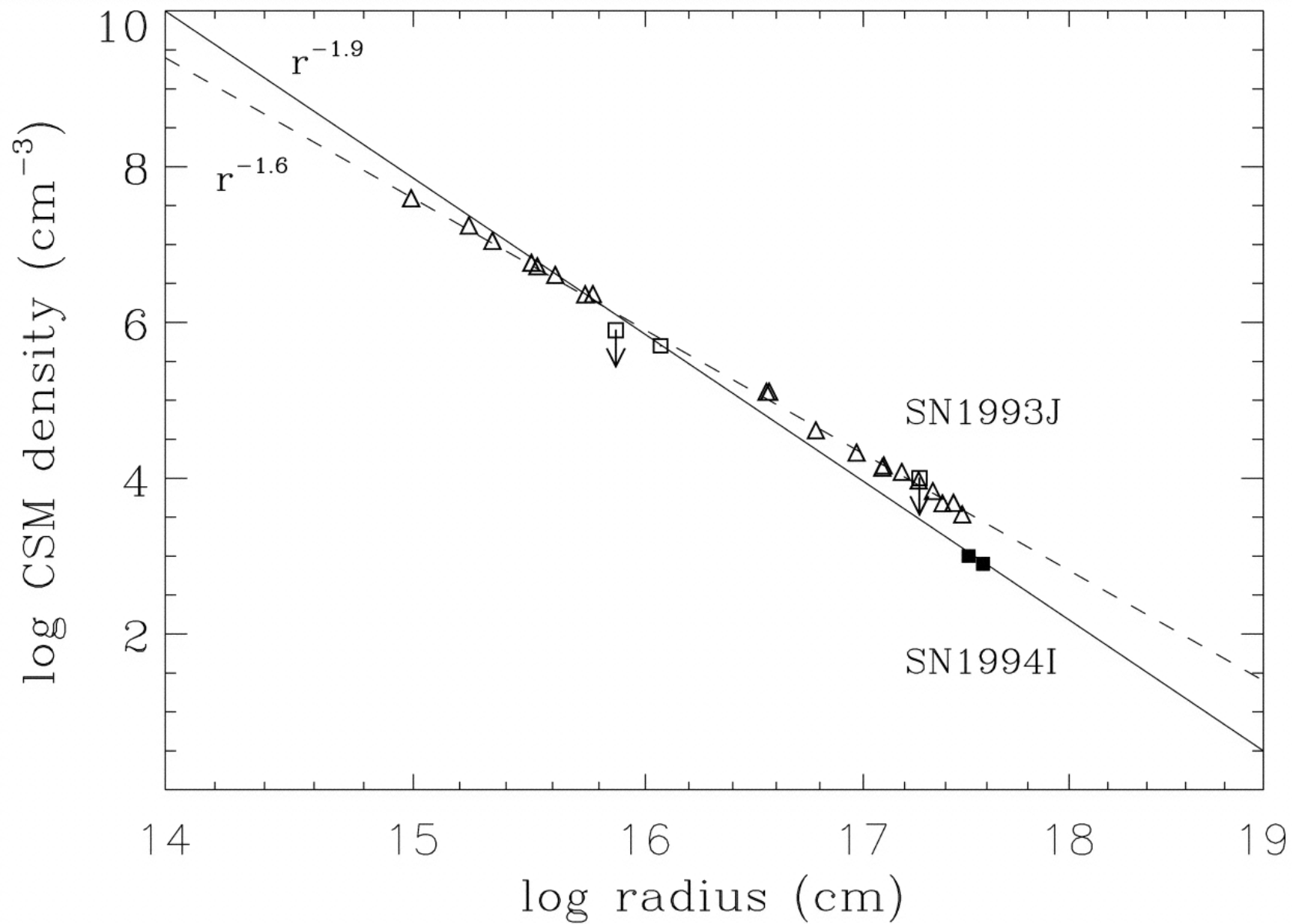
Fig. 3. from XRay Emission from the Type Ic Supernova 1994I Observed with Chandra Immler, Wilson, & Terashima 2002 ApJL 573 L27 doi:10.1086/341935 https://dx.doi.org/10.1086/341935 © 2002. The American Astronomical Society. All rights reserved. Printed in U.S.A.
