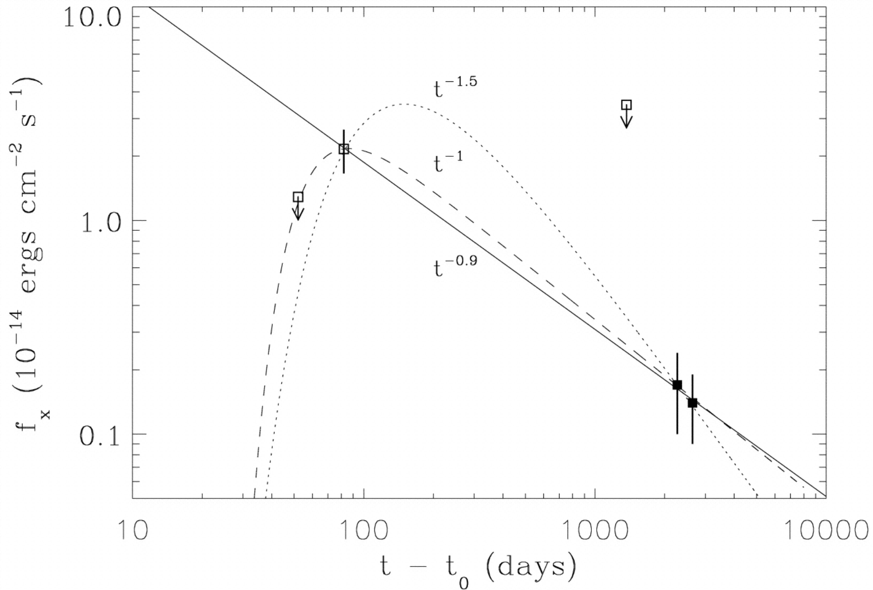
Fig. 2. from XRay Emission from the Type Ic Supernova 1994I Observed with Chandra Immler, Wilson, & Terashima 2002 ApJL 573 L27 doi:10.1086/341935 https://dx.doi.org/10.1086/341935 © 2002. The American Astronomical Society. All rights reserved. Printed in U.S.A.
