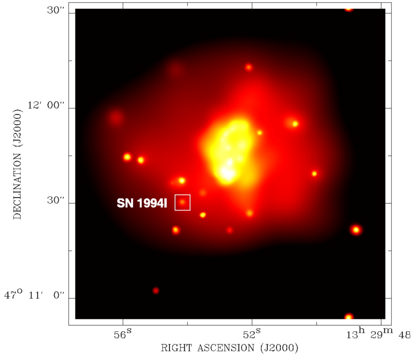
Fig. 1. from XRay Emission from the Type Ic Supernova 1994I Observed with Chandra Immler, Wilson, & Terashima 2002 ApJL 573 L27 doi:10.1086/341935 https://dx.doi.org/10.1086/341935 © 2002. The American Astronomical Society. All rights reserved. Printed in U.S.A.
