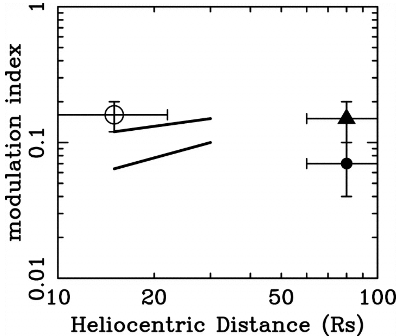
Fig. 2. from The Amplitude of Magnetohydrodynamic Turbulence in the Inner Solar Wind Spangler 2002 ApJ 576 997 doi:10.1086/341889 https://dx.doi.org/10.1086/341889 © 2002. The American Astronomical Society. All rights reserved. Printed in U.S.A.
