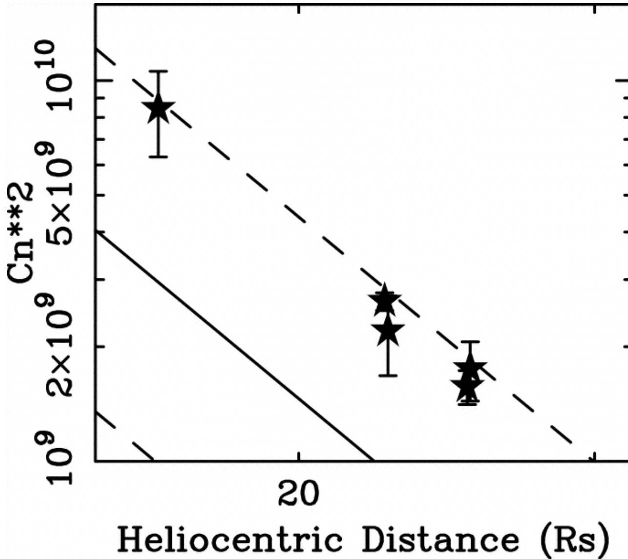
Fig. 1. from The Amplitude of Magnetohydrodynamic Turbulence in the Inner Solar Wind Spangler 2002 ApJ 576 997 doi:10.1086/341889 https://dx.doi.org/10.1086/341889 © 2002. The American Astronomical Society. All rights reserved. Printed in U.S.A.
