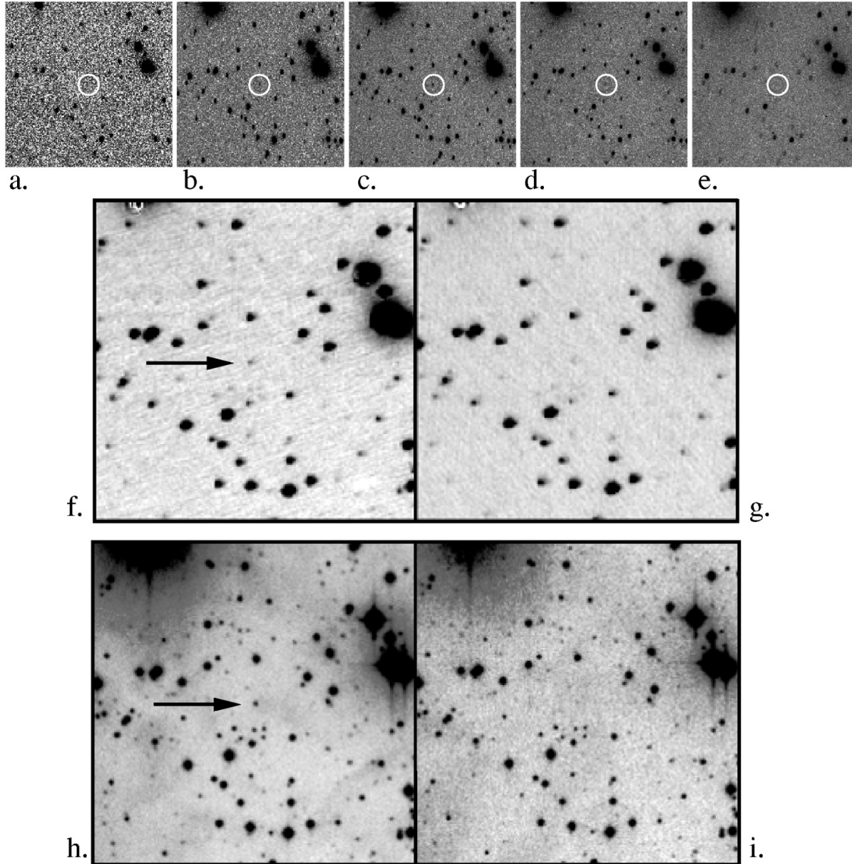
Fig. 1. from LOTIS, SuperLOTIS, Sloan Digital Sky Survey, and Tautenburg Observations of GRB 010921 Park et al. 2002 ApJL 571 L131 doi:10.1086/341334 https://dx.doi.org/10.1086/341334
