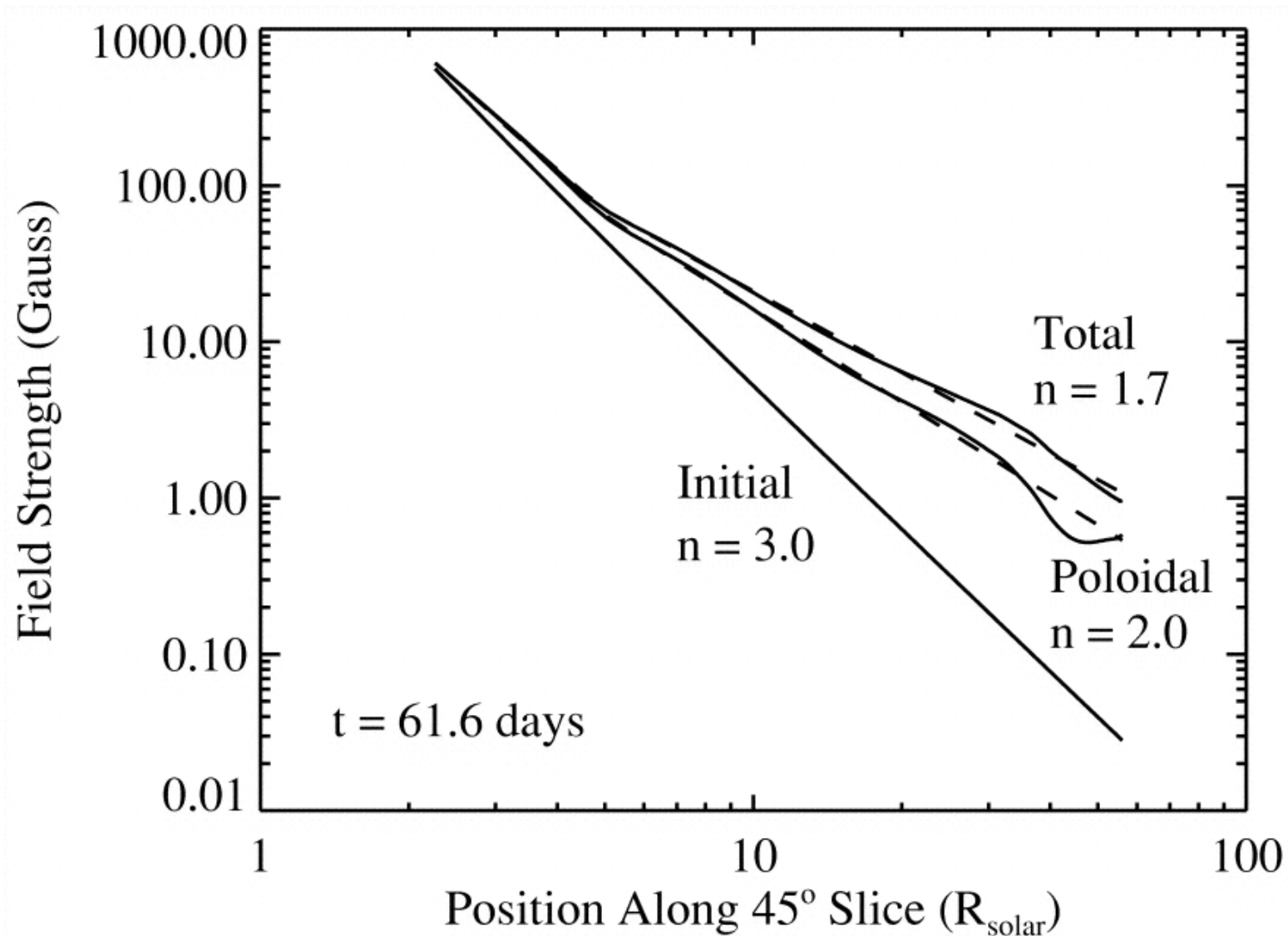
Fig. 8. from Simulationbased Investigation of a Model for the Interaction between Stellar Magnetospheres and Circumstellar Accretion Disks Matt et al. 2002 ApJ 574 232 doi:10.1086/340896 https://dx.doi.org/10.1086/340896 © 2002. The American Astronomical Society. All rights reserved. Printed in U.S.A.
