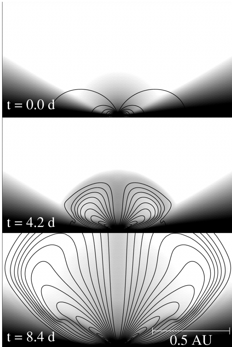
Fig. 7. from Simulationbased Investigation of a Model for the Interaction between Stellar Magnetospheres and Circumstellar Accretion Disks Matt et al. 2002 ApJ 574 232 doi:10.1086/340896 https://dx.doi.org/10.1086/340896 © 2002. The American Astronomical Society. All rights reserved. Printed in U.S.A.
