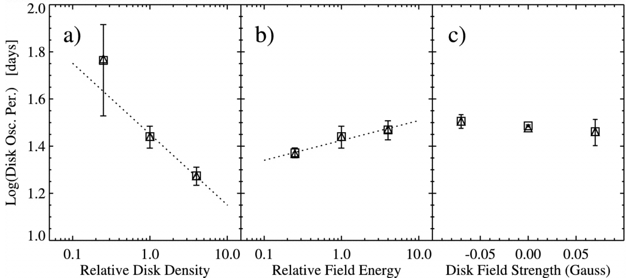
Fig. 12. from Simulationbased Investigation of a Model for the Interaction between Stellar Magnetospheres and Circumstellar Accretion Disks Matt et al. 2002 ApJ 574 232 doi:10.1086/340896 https://dx.doi.org/10.1086/340896 © 2002. The American Astronomical Society. All rights reserved. Printed in U.S.A.
