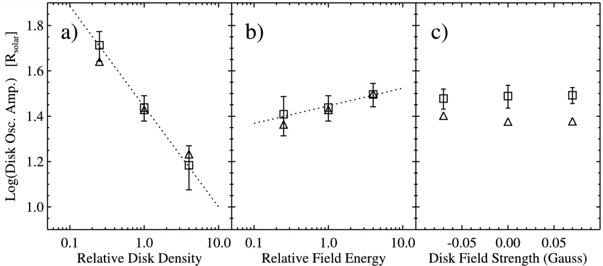
Fig. 11. from Simulationbased Investigation of a Model for the Interaction between Stellar Magnetospheres and Circumstellar Accretion Disks Matt et al. 2002 ApJ 574 232 doi:10.1086/340896 https://dx.doi.org/10.1086/340896 © 2002. The American Astronomical Society. All rights reserved. Printed in U.S.A.
