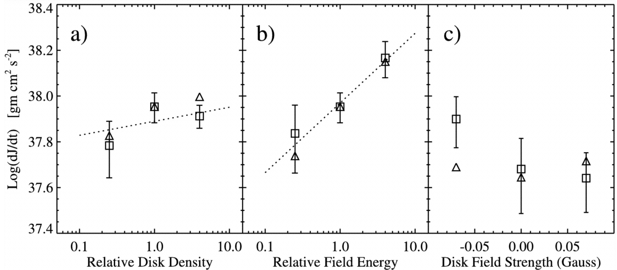
Fig. 10. from Simulationbased Investigation of a Model for the Interaction between Stellar Magnetospheres and Circumstellar Accretion Disks Matt et al. 2002 ApJ 574 232 doi:10.1086/340896 https://dx.doi.org/10.1086/340896 © 2002. The American Astronomical Society. All rights reserved. Printed in U.S.A.
