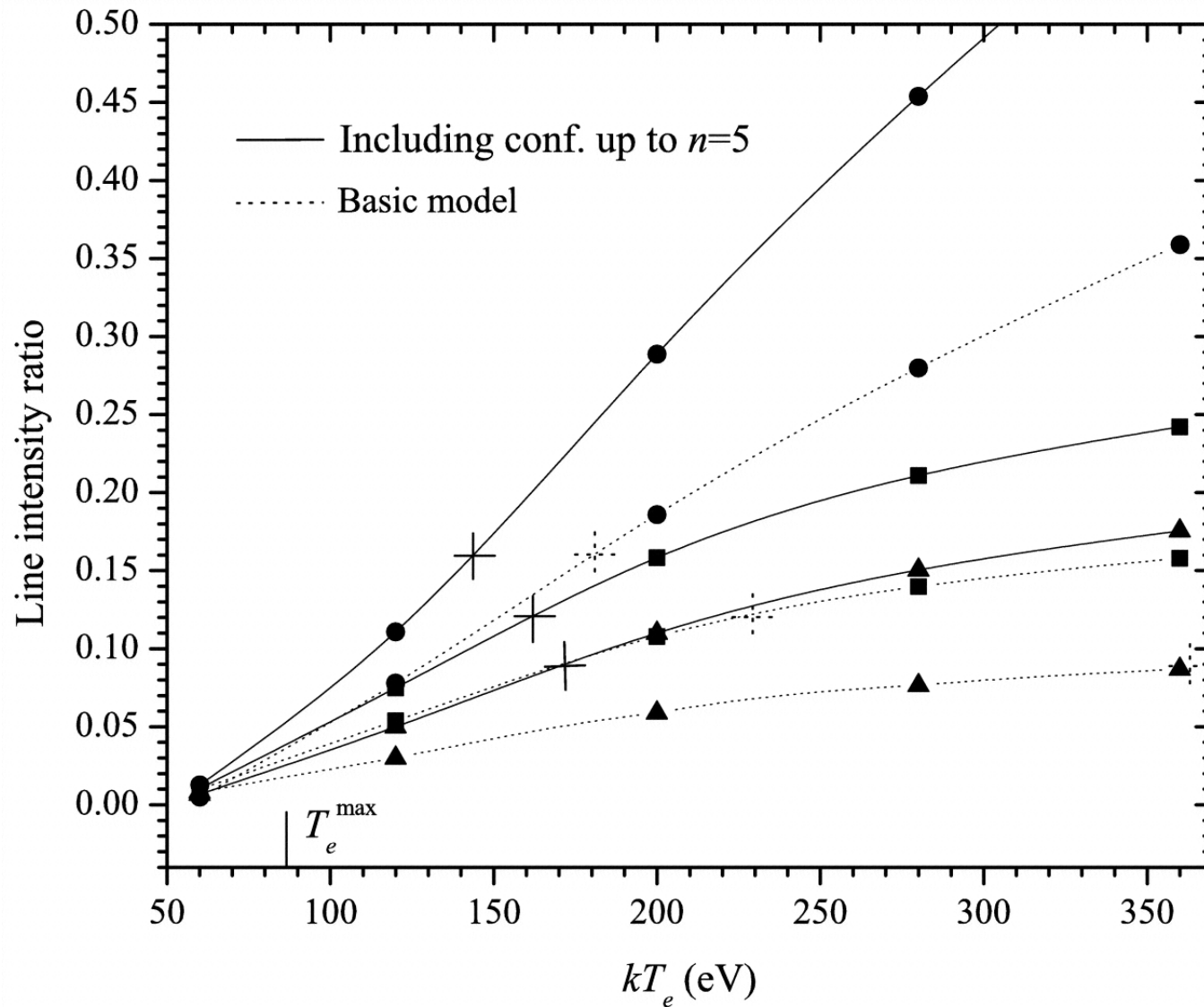
Fig. 3. from The Effect of Highlylying Levels on Atomic Models Relevant to Spectroscopic Analyses of Solar ExtremeUltraviolet Spectra Doron et al. 2002 ApJ 574 504 doi:10.1086/340839 https://dx.doi.org/10.1086/340839 © 2002. The American Astronomical Society. All rights reserved. Printed in U.S.A.
