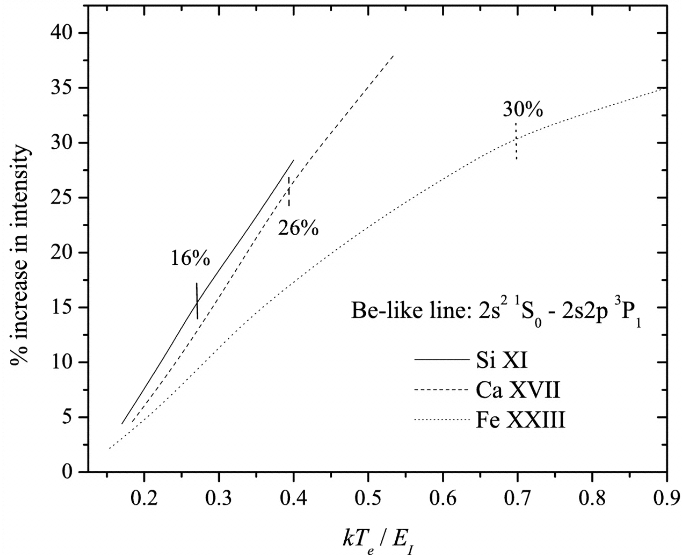
Fig. 2. from The Effect of Highlylying Levels on Atomic Models Relevant to Spectroscopic Analyses of Solar ExtremeUltraviolet Spectra Doron et al. 2002 ApJ 574 504 doi:10.1086/340839 https://dx.doi.org/10.1086/340839 © 2002. The American Astronomical Society. All rights reserved. Printed in U.S.A.
