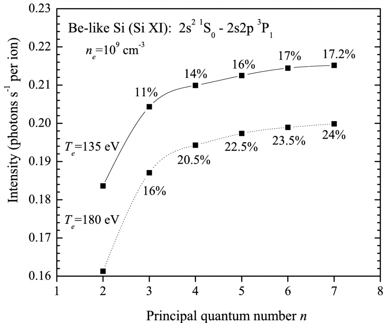
Fig. 1. from The Effect of Highlylying Levels on Atomic Models Relevant to Spectroscopic Analyses of Solar ExtremeUltraviolet Spectra Doron et al. 2002 ApJ 574 504 doi:10.1086/340839 https://dx.doi.org/10.1086/340839 © 2002. The American Astronomical Society. All rights reserved. Printed in U.S.A.
