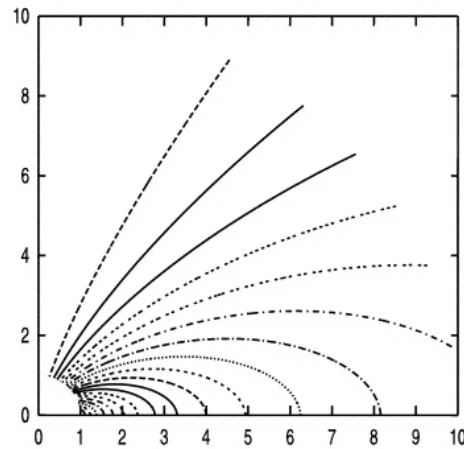
Fig. 2. from Partial Field Opening and Current Sheet Formation in the Disk Magnetosphere Uzdensky 2002 ApJ 572 432 doi:10.1086/340308 https://dx.doi.org/10.1086/340308 © 2002. The American Astronomical Society. All rights reserved. Printed in U.S.A.
