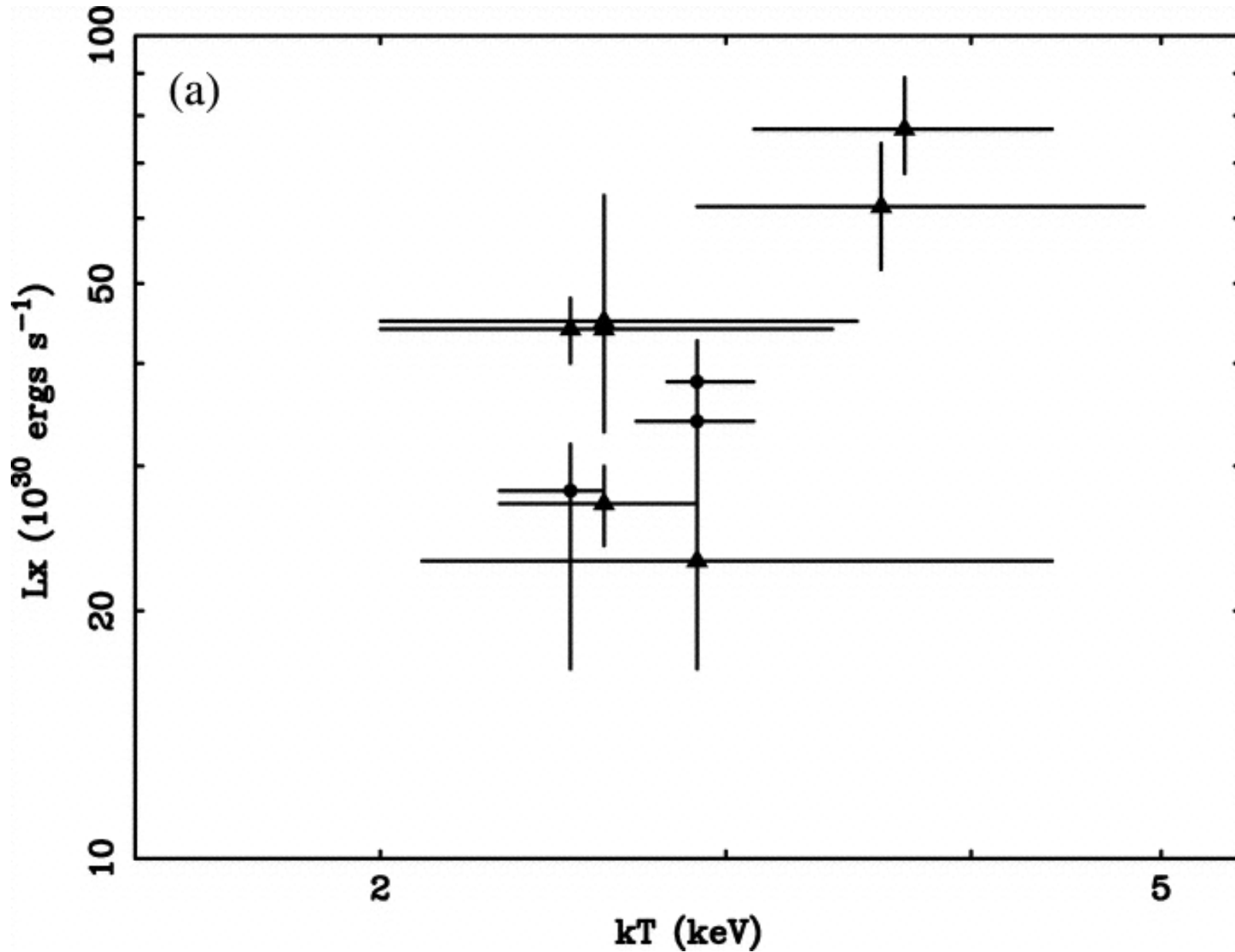
Fig. 6. from Chandra and ASCA Observations of the XRay–brightest T Tauri Stars in the Ophiuchi Cloud Imanishi, Tsujimoto, & Koyama 2002 ApJ 572 300 doi:10.1086/340306 https://dx.doi.org/10.1086/340306 © 2002. The American Astronomical Society. All rights reserved. Printed in U.S.A.
