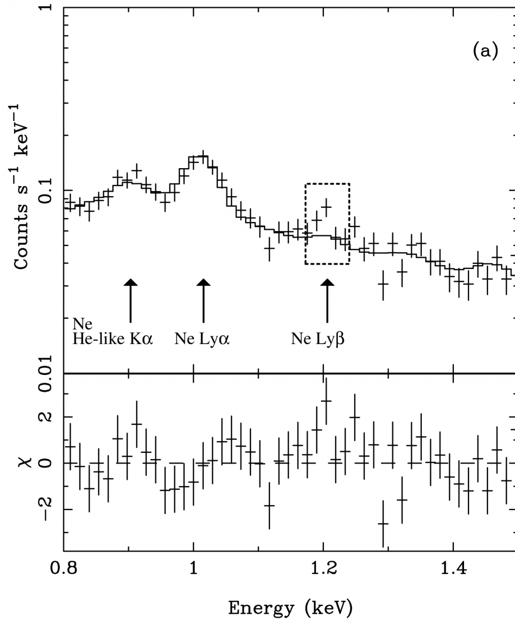
Fig. 5. from Chandra and ASCA Observations of the XRay–brightest T Tauri Stars in the Ophiuchi Cloud Imanishi, Tsujimoto, & Koyama 2002 ApJ 572 300 doi:10.1086/340306 https://dx.doi.org/10.1086/340306
