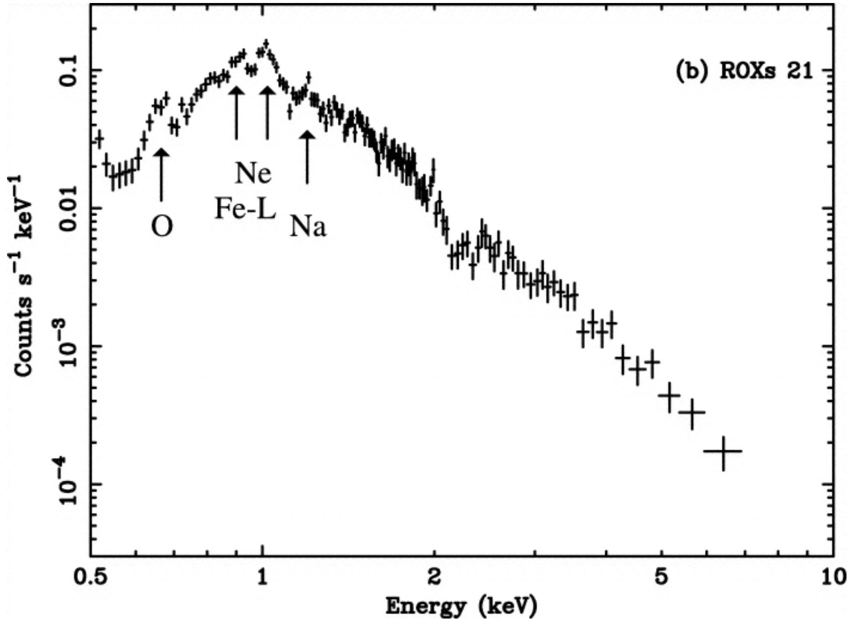
Fig. 3. from Chandra and ASCA Observations of the XRay–brightest T Tauri Stars in the Ophiuchi Cloud Imanishi, Tsujimoto, & Koyama 2002 ApJ 572 300 doi:10.1086/340306 https://dx.doi.org/10.1086/340306 © 2002. The American Astronomical Society. All rights reserved. Printed in U.S.A.
