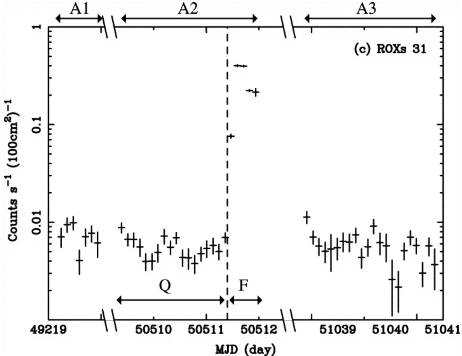
Fig. 2. from Chandra and ASCA Observations of the XRay–brightest T Tauri Stars in the Ophiuchi Cloud Imanishi, Tsujimoto, & Koyama 2002 ApJ 572 300 doi:10.1086/340306 https://dx.doi.org/10.1086/340306
