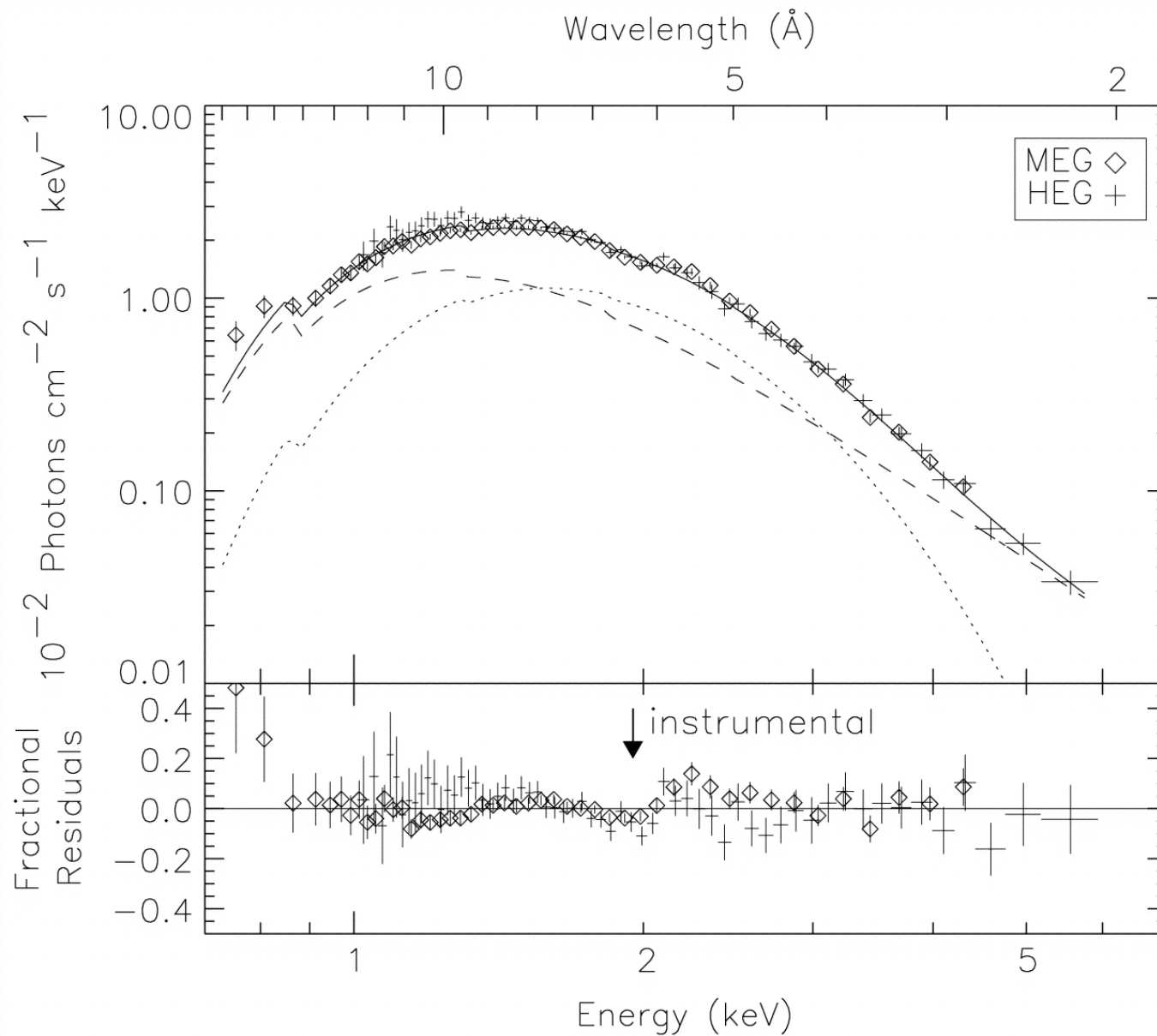
Fig. 1. from Chandra HighResolution Spectrum of the Anomalous XRay Pulsar 4U 0142+61 Juett et al. 2002 ApJL 568 L31 doi:10.1086/340273 https://dx.doi.org/10.1086/340273 © 2002. The American Astronomical Society. All rights reserved. Printed in U.S.A.
