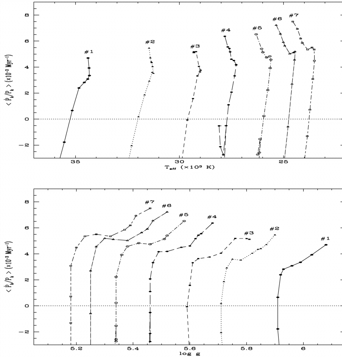
Fig. 8. from Adiabatic Survey of Subdwarf B Star Oscillations. III. Effects of Extreme Horizontal Branch Stellar Evolution on Pulsation Modes Charpinet et al. 2002 ApJS 140 469 doi:10.1086/339707 https://dx.doi.org/10.1086/339707
