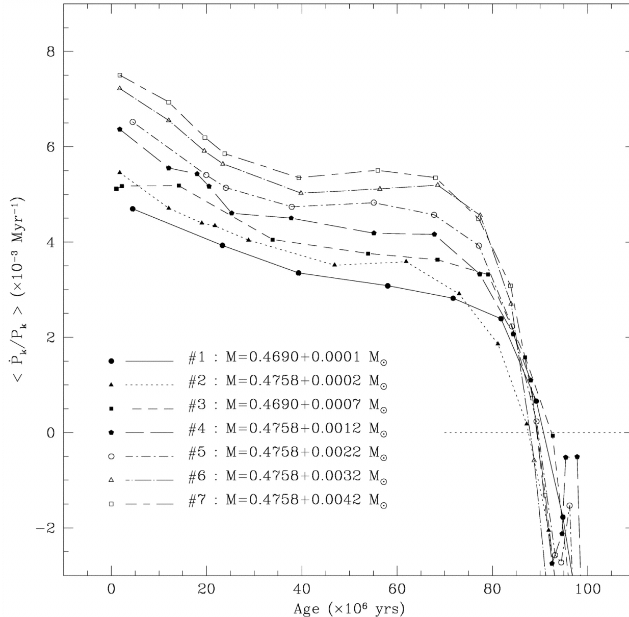
Fig. 7. from Adiabatic Survey of Subdwarf B Star Oscillations. III. Effects of Extreme Horizontal Branch Stellar Evolution on Pulsation Modes Charpinet et al. 2002 ApJS 140 469 doi:10.1086/339707 https://dx.doi.org/10.1086/339707 © 2002. The American Astronomical Society. All rights reserved. Printed in U.S.A.
