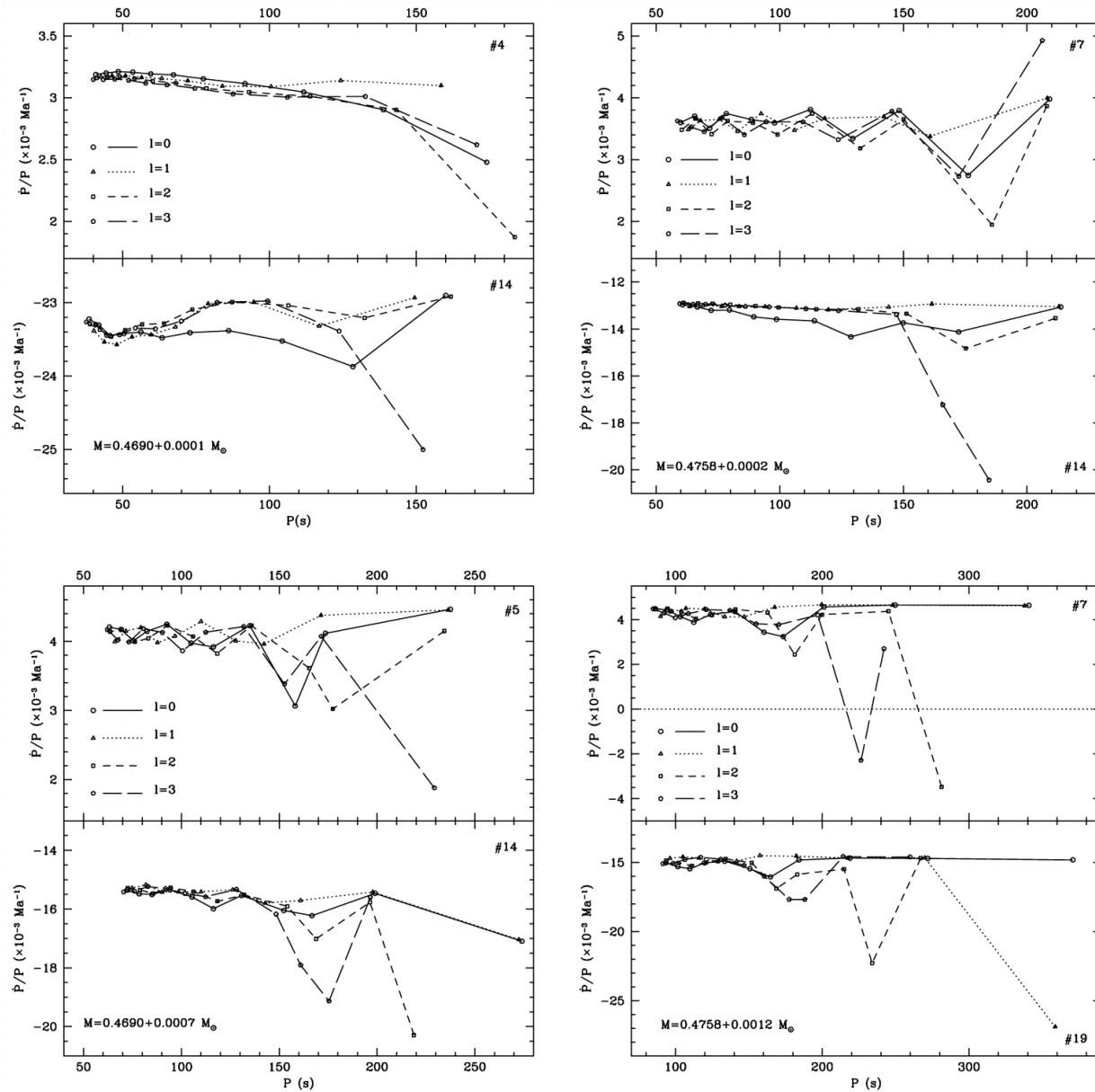
Fig. 5. from Adiabatic Survey of Subdwarf B Star Oscillations. III. Effects of Extreme Horizontal Branch Stellar Evolution on Pulsation Modes Charpinet et al. 2002 ApJS 140 469 doi:10.1086/339707 https://dx.doi.org/10.1086/339707
