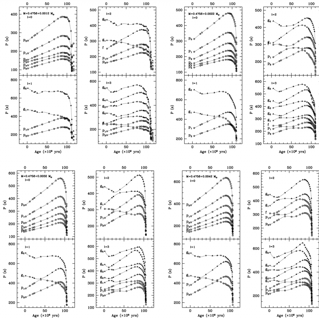
Fig. 3. from Adiabatic Survey of Subdwarf B Star Oscillations. III. Effects of Extreme Horizontal Branch Stellar Evolution on Pulsation Modes Charpinet et al. 2002 ApJS 140 469 doi:10.1086/339707 https://dx.doi.org/10.1086/339707
