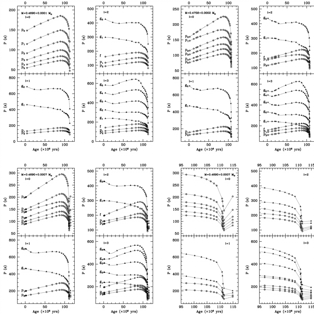
Fig. 2. from Adiabatic Survey of Subdwarf B Star Oscillations. III. Effects of Extreme Horizontal Branch Stellar Evolution on Pulsation Modes Charpinet et al. 2002 ApJS 140 469 doi:10.1086/339707 https://dx.doi.org/10.1086/339707
