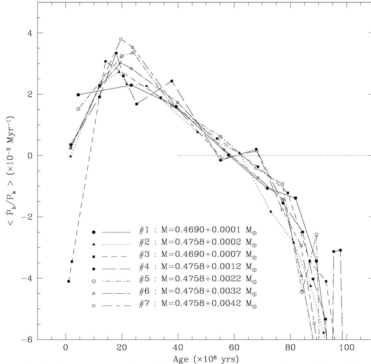
Fig. 12. from Adiabatic Survey of Subdwarf B Star Oscillations. III. Effects of Extreme Horizontal Branch Stellar Evolution on Pulsation Modes Charpinet et al. 2002 ApJS 140 469 doi:10.1086/339707 https://dx.doi.org/10.1086/339707 © 2002. The American Astronomical Society. All rights reserved. Printed in U.S.A.
