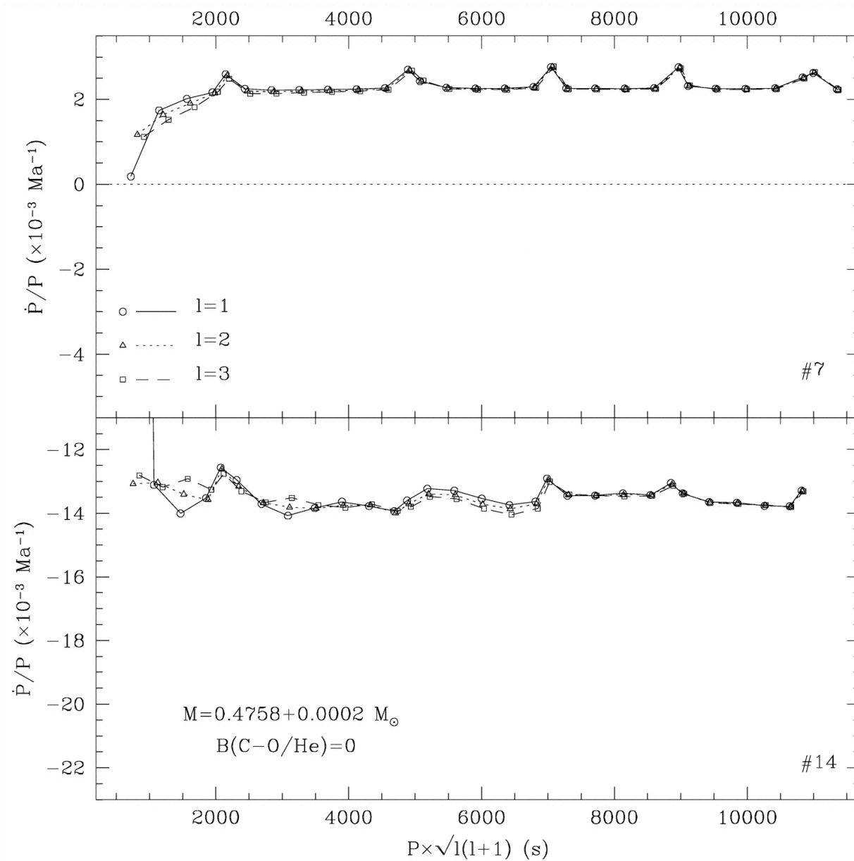
Fig. 11. from Adiabatic Survey of Subdwarf B Star Oscillations. III. Effects of Extreme Horizontal Branch Stellar Evolution on Pulsation Modes Charpinet et al. 2002 ApJS 140 469 doi:10.1086/339707 https://dx.doi.org/10.1086/339707
