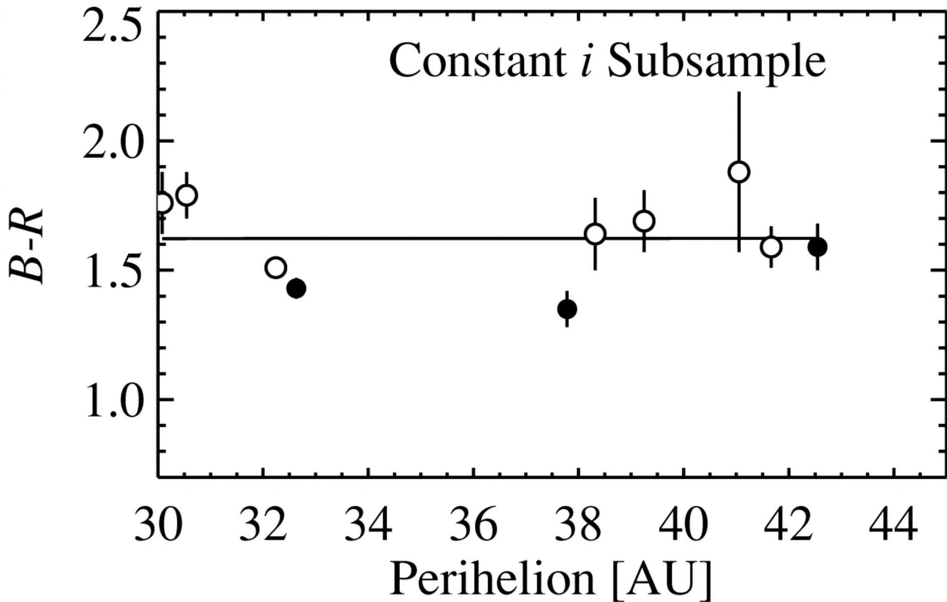
Fig. 3. from A Correlation between Inclination and Color in the Classical Kuiper Belt Trujillo & Brown 2002 ApJL 566 L125 doi:10.1086/339437 https://dx.doi.org/10.1086/339437 © 2002. The American Astronomical Society. All rights reserved. Printed in U.S.A.
