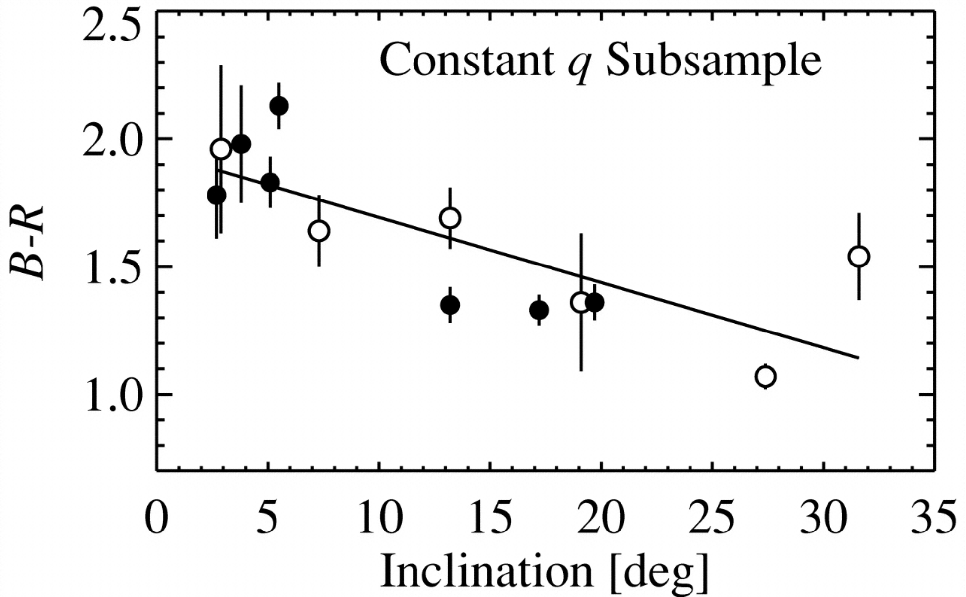
Fig. 3. from A Correlation between Inclination and Color in the Classical Kuiper Belt Trujillo & Brown 2002 ApJL 566 L125 doi:10.1086/339437 https://dx.doi.org/10.1086/339437 © 2002. The American Astronomical Society. All rights reserved. Printed in U.S.A.
