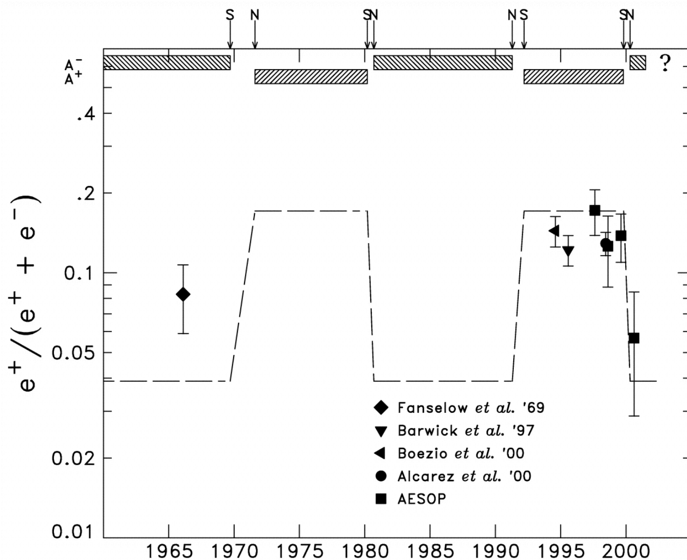
Fig. 5. from Positron Abundance in Galactic Cosmic Rays Clem & Evenson 2002 ApJ 568 216 doi:10.1086/338841 https://dx.doi.org/10.1086/338841 © 2002. The American Astronomical Society. All rights reserved. Printed in U.S.A.
