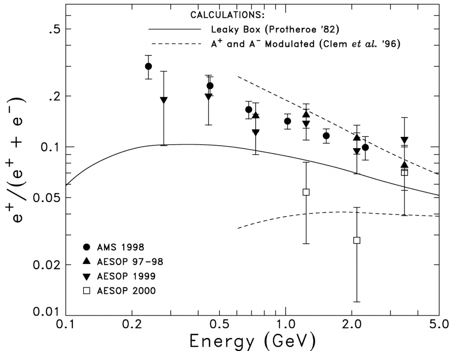
Fig. 4. from Positron Abundance in Galactic Cosmic Rays Clem & Evenson 2002 ApJ 568 216 doi:10.1086/338841 https://dx.doi.org/10.1086/338841 © 2002. The American Astronomical Society. All rights reserved. Printed in U.S.A.
