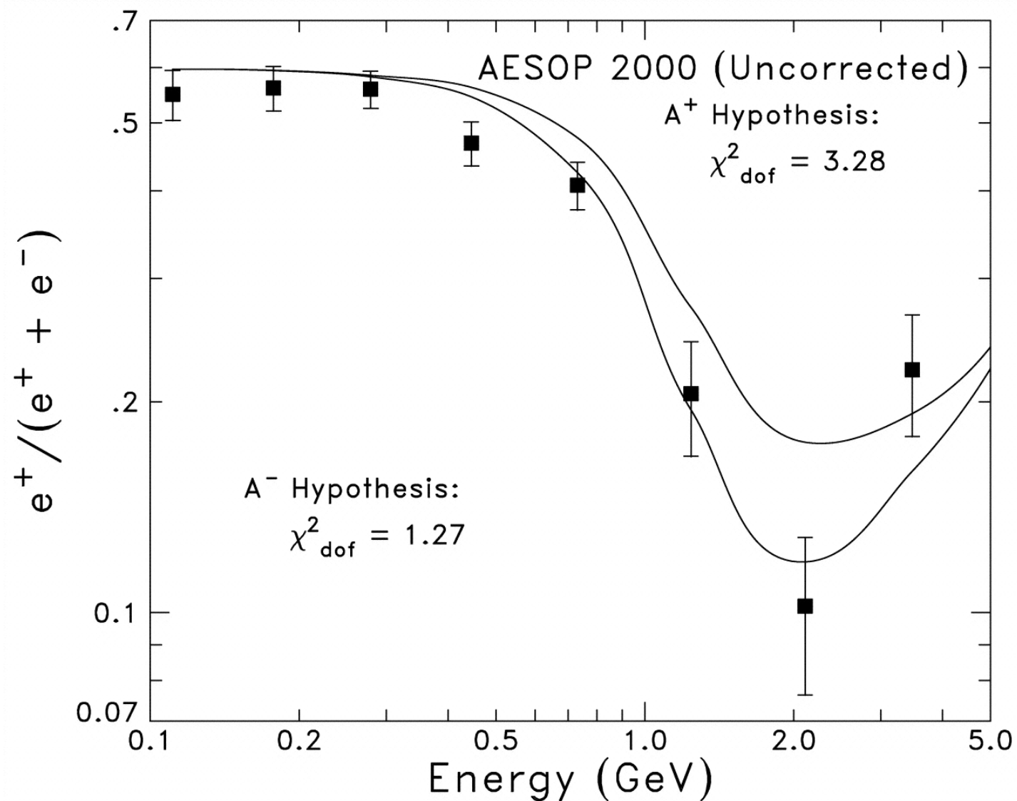
Fig. 3. from Positron Abundance in Galactic Cosmic Rays Clem & Evenson 2002 ApJ 568 216 doi:10.1086/338841 https://dx.doi.org/10.1086/338841 © 2002. The American Astronomical Society. All rights reserved. Printed in U.S.A.
