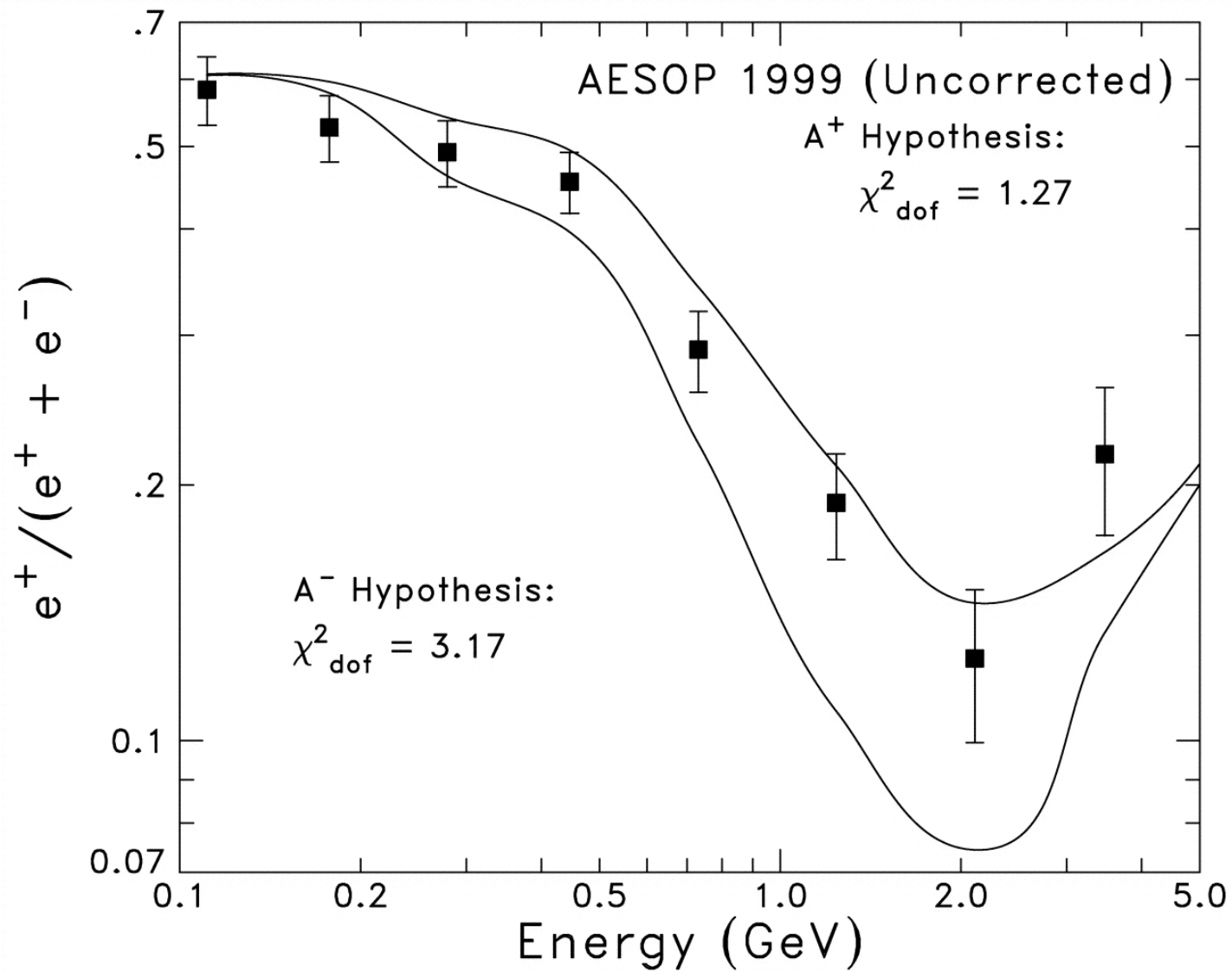
Fig. 2. from Positron Abundance in Galactic Cosmic Rays Clem & Evenson 2002 ApJ 568 216 doi:10.1086/338841 https://dx.doi.org/10.1086/338841 © 2002. The American Astronomical Society. All rights reserved. Printed in U.S.A.
