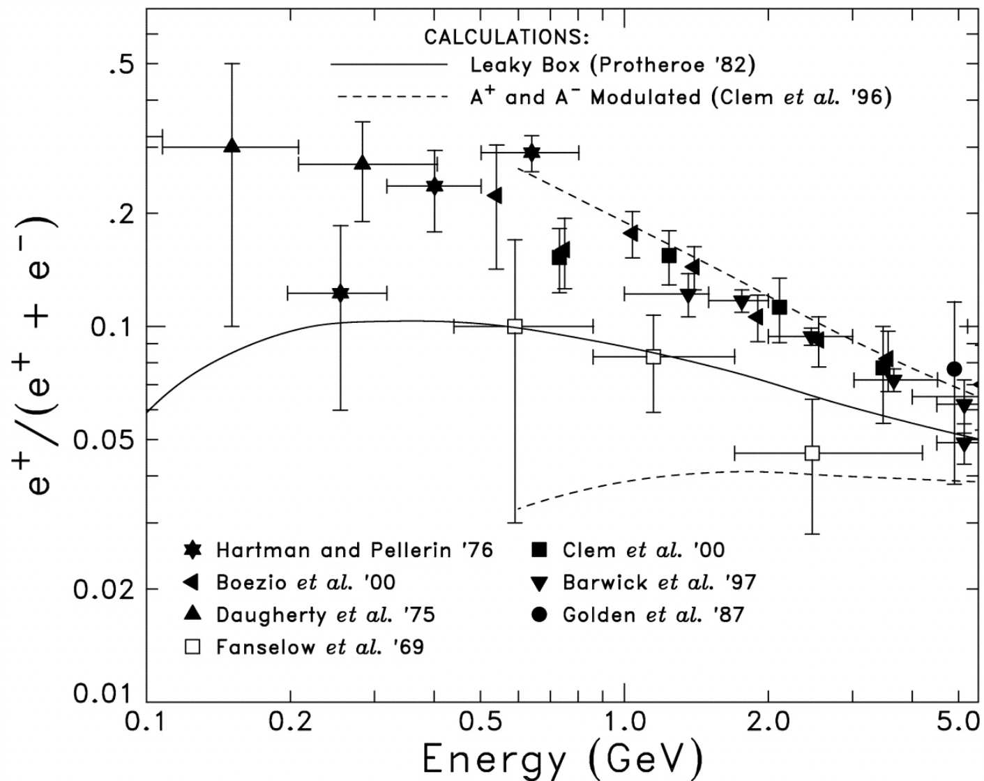
Fig. 1. from Positron Abundance in Galactic Cosmic Rays Clem & Evenson 2002 ApJ 568 216 doi:10.1086/338841 https://dx.doi.org/10.1086/338841 © 2002. The American Astronomical Society. All rights reserved. Printed in U.S.A.
