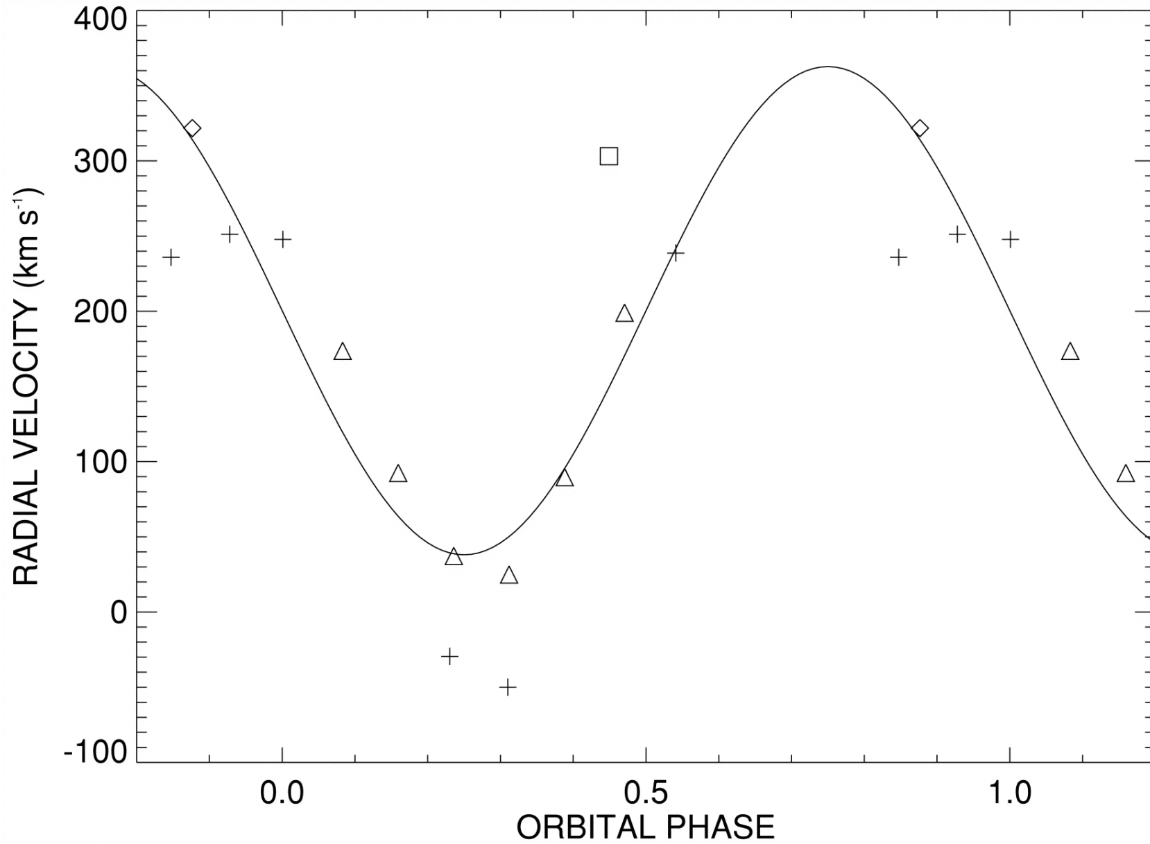
Fig. 9. from The Spectral Components of SS 433 Gies et al. 2002 ApJ 566 1069 doi:10.1086/338335 https://dx.doi.org/10.1086/338335
