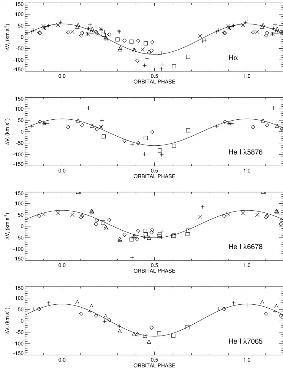
Fig. 8. from The Spectral Components of SS 433 Gies et al. 2002 ApJ 566 1069 doi:10.1086/338335 https://dx.doi.org/10.1086/338335
