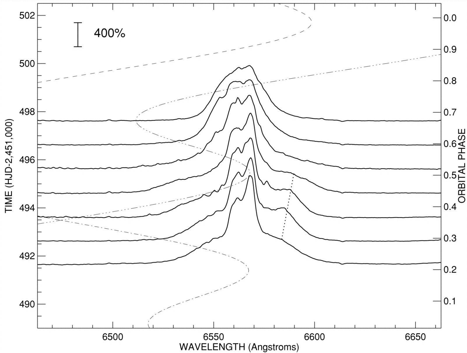
Fig. 7. from The Spectral Components of SS 433 Gies et al. 2002 ApJ 566 1069 doi:10.1086/338335 https://dx.doi.org/10.1086/338335
